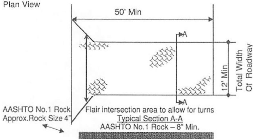
Plan View
