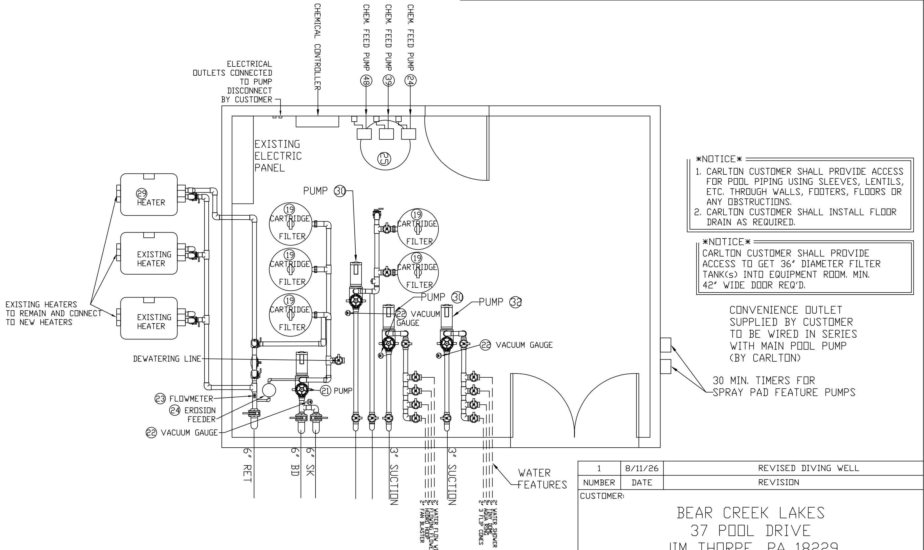
FILTER ROOM SCALE: 3/8" = 1'-0"
